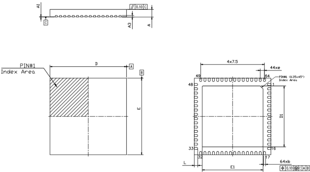
Figure 4: QFN64 Package
